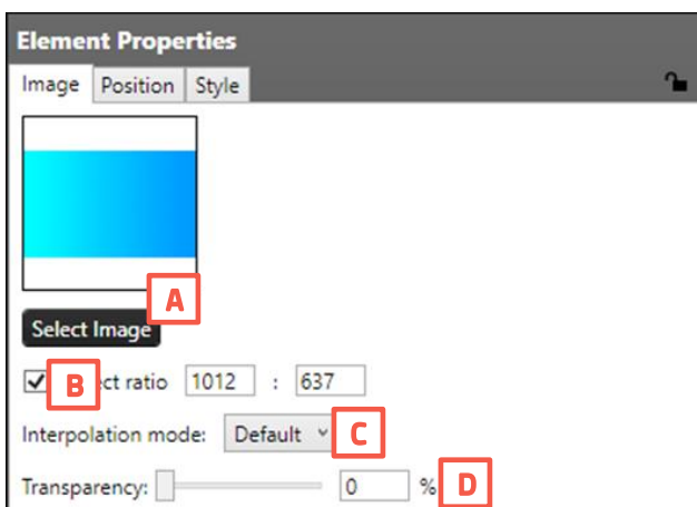
Fig. Example of the Image element properties
